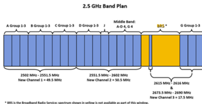
Figure 2.1: 2.5 GHz Band Plan 10
